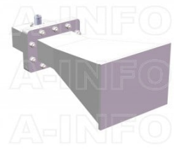
LB-340-10-C-NFSPO Standard Gain Horn Antenna 2.2-3.3GHz 10dB Gain N Type Female
