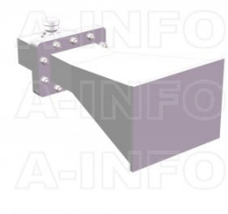
LB-340-10-C-7/16FSP Standard Gain Horn Antenna 2.2-3.3GHz 10dB Gain 7/16(DIN) Female
